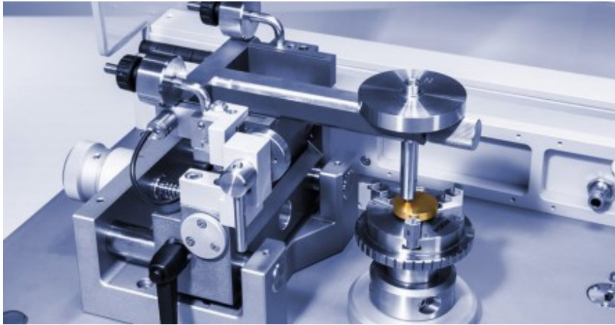
Fig. 4.16: The tribometer used for the wear test [20]
