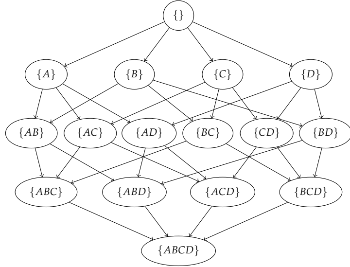
FIGURE 3.1: parent set lattice for 4 variables.
