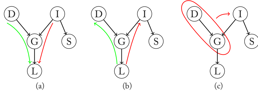
FIGURE 2.1: example of flows of influence in a Bayesian Network. Examples taken from https://class.coursera.org/pgm-003/ .
