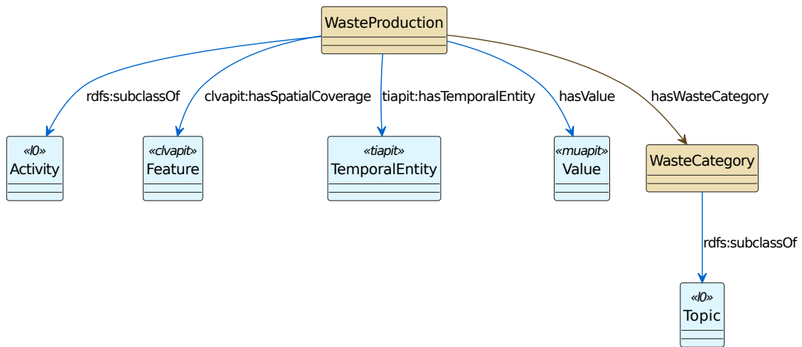
Figure 5.9: Waste Production semantic area.
