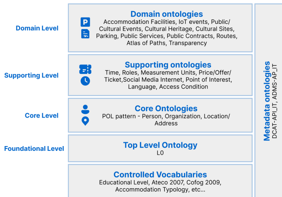
Figure 2.8: The OntoPiA ontological stack.
