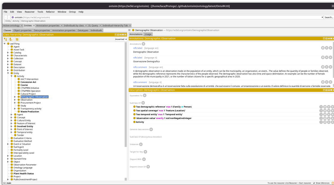
Figure 2.4: A snapshot of the Protégé "Entities" tab.
