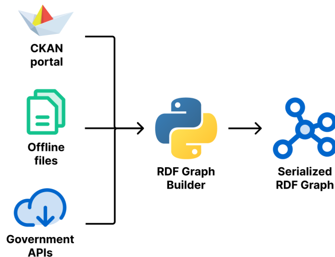
Figure 6.1: RDF Graph Builder architecture.
