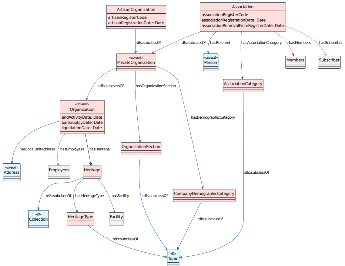
Figure 5.3: Organizations and Associations semantic area.
