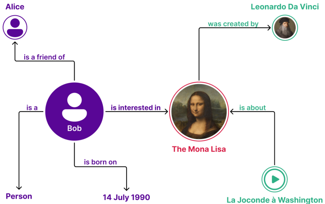
Figure 2.2: The example of the RDF Graph presented by W3C.
