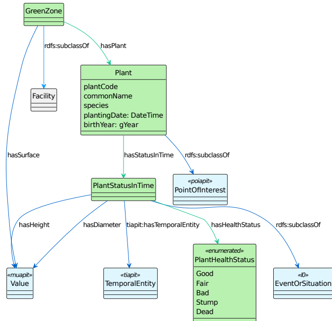
Figure 5.7: Green Zones and Plants semantic area.
