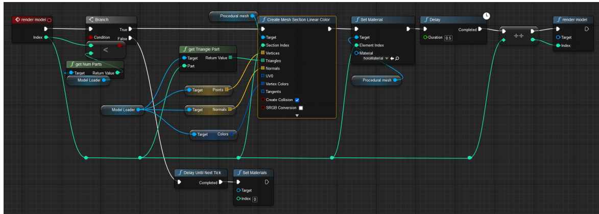
Figure 4.1: Loading mesh function
