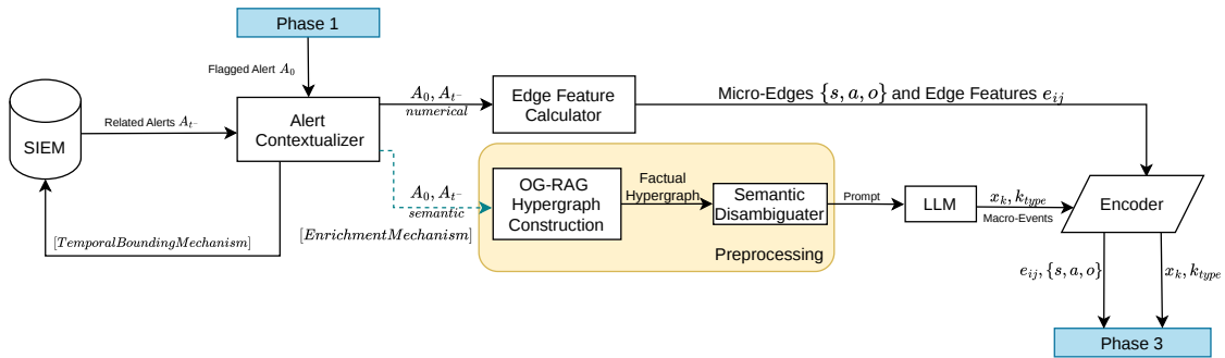
Figure 2: Phase 2 Architecture mapping the transformation of raw SIEM alerts
