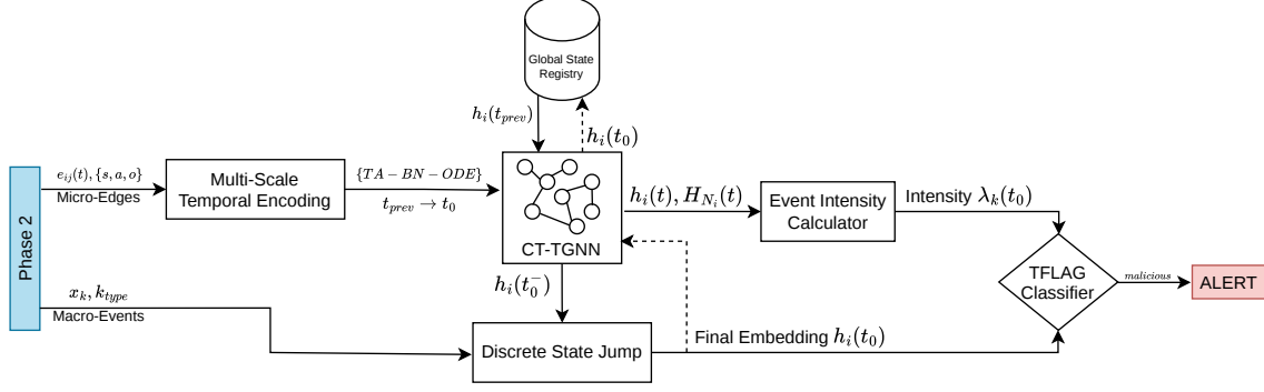
Figure 3: The Phase 3 Architecture routing continuous and discrete payloads through the CT-TGNN to Alert
