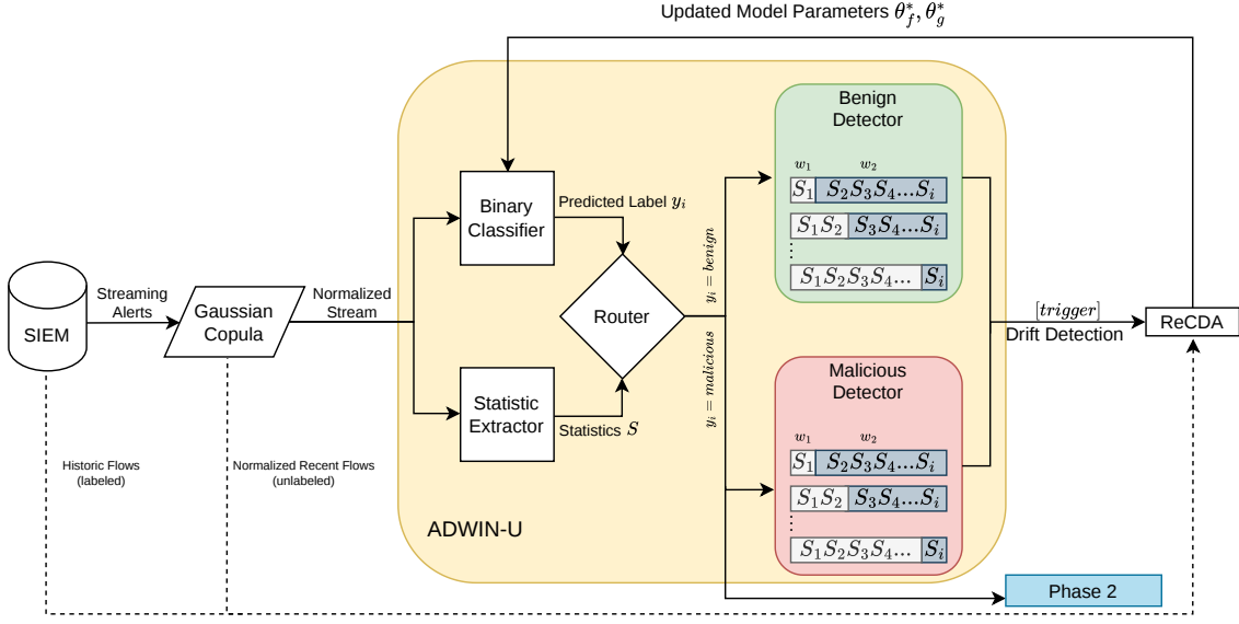
Figure 1: Phase 1 Architecture for continuous drift detection & mitigation
