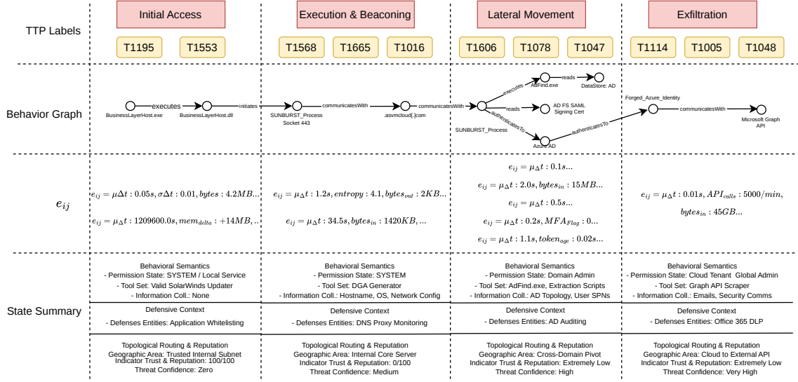
Figure 4: Dry-Run of the SolarWinds Attack represented in modified AttackKG+ Structure
