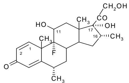
Fluorometolone
