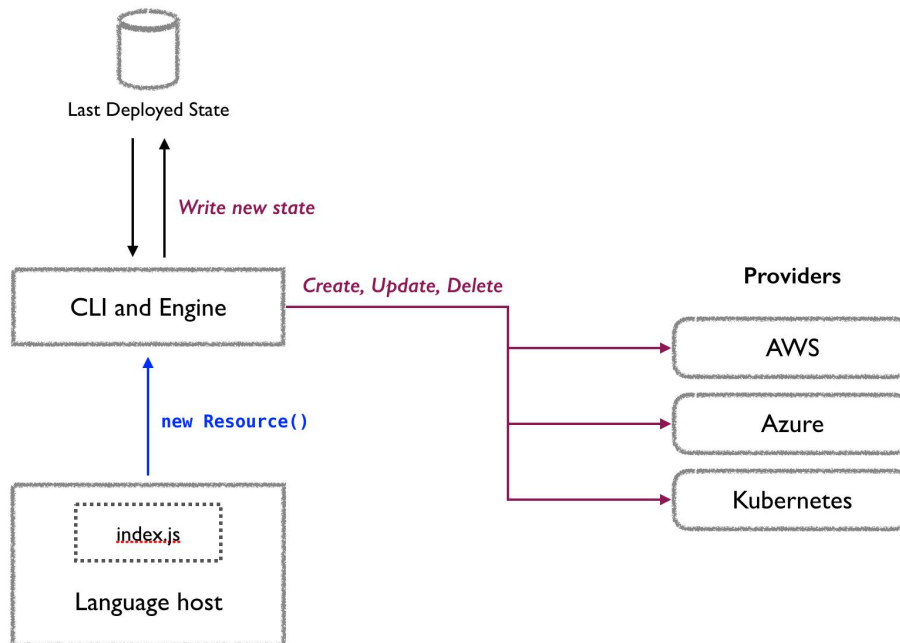
Image 3.1: Pulumi architecture
