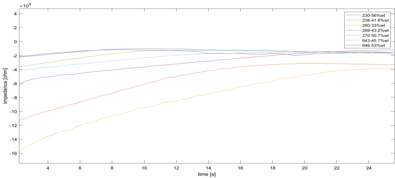
Fig.35 Impedance comparison
