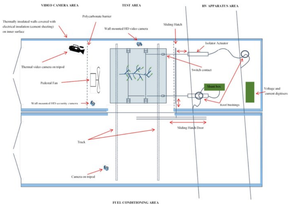
Fig.22 Test layout
