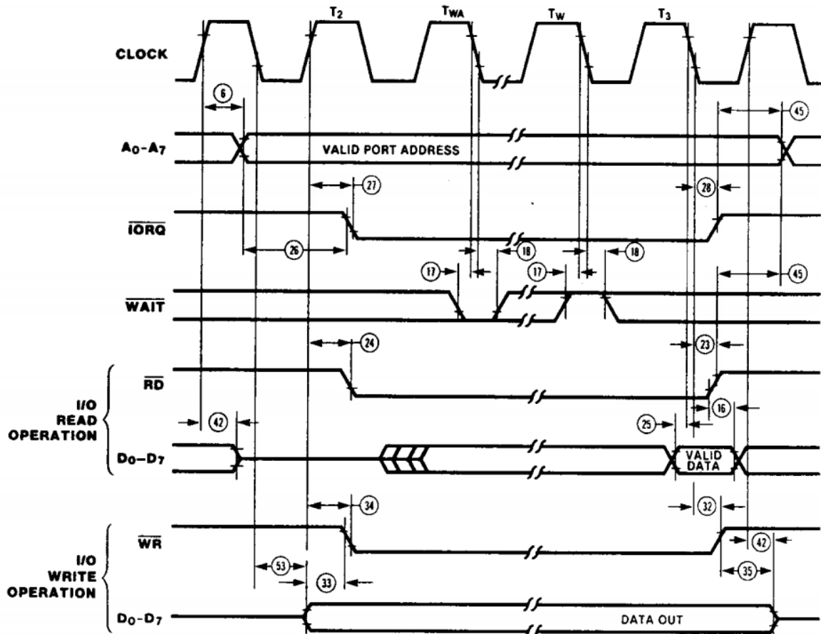
FIGURA 3-34 - INPUT OR OUTPUT CYCLES [19]
