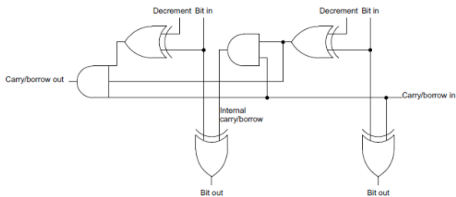
FIGURA 3-14 -CELLA INC/DEC A 2 BIT BASE [27]
