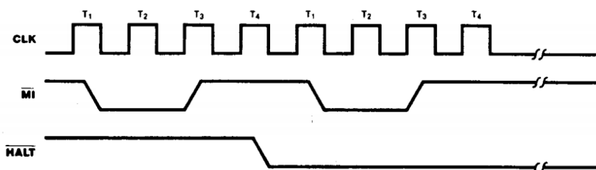
FIGURA 3-24 - POWER-DOWN ACKNOWLEDGE [19]
