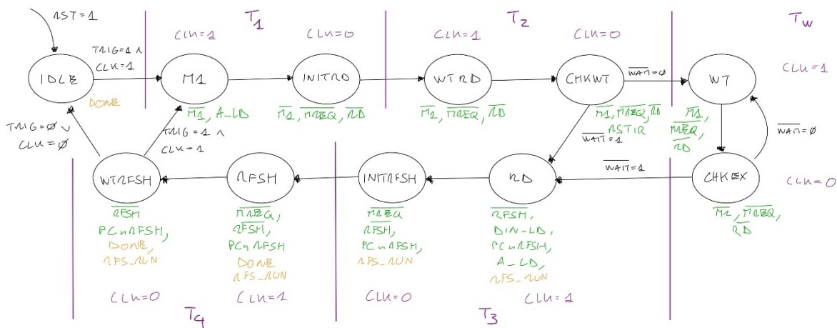
FIGURA 3-29 - INSTRUCTION OPCODE FETCH [19]
