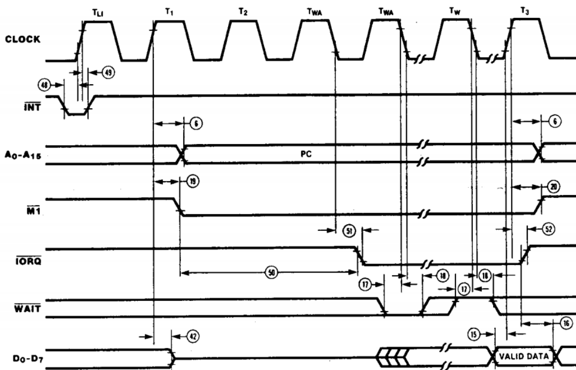
FIGURA 3-35 - INTERRUPT REQUEST/ACKNOWLEDGE CYCLE [19]
