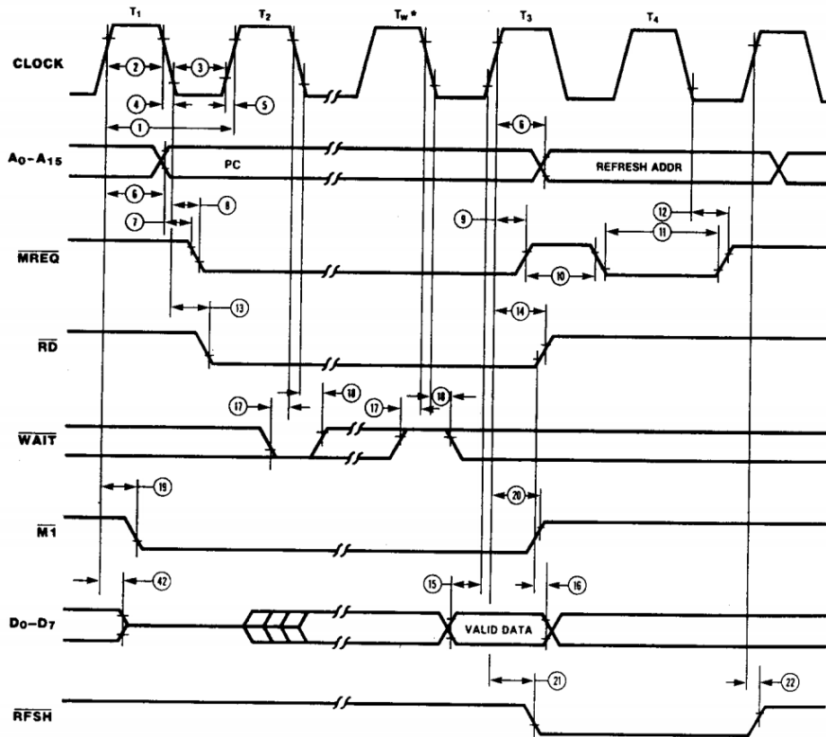
FIGURA 3-29 - INSTRUCTION OPCODE FETCH [19]
