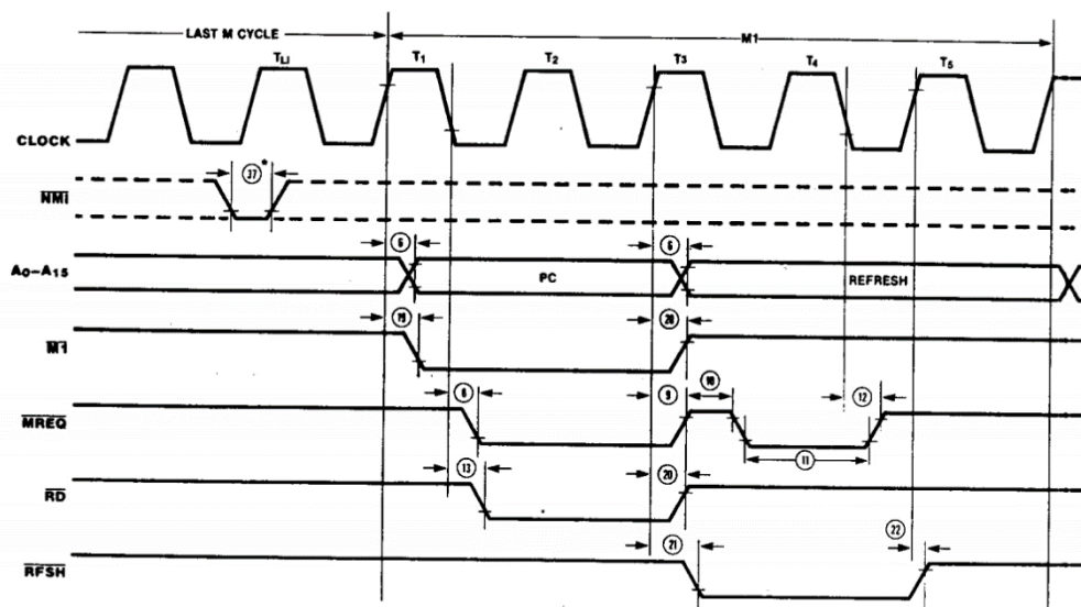
FIGURA 3-26 - NON-MASKABLE INTERRUPT REQUEST OPERATION [19]
