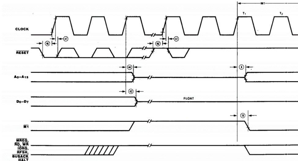
FIGURA 3-27 - RESET CYCLE [19]
