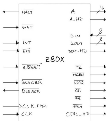
FIGURA 3-16 - PINOUT ENTITY Z80
