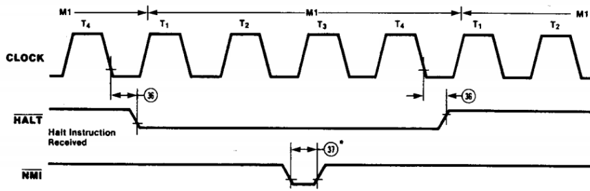
FIGURA 3-23 - HALT ACKNOWLEDGE [19]
