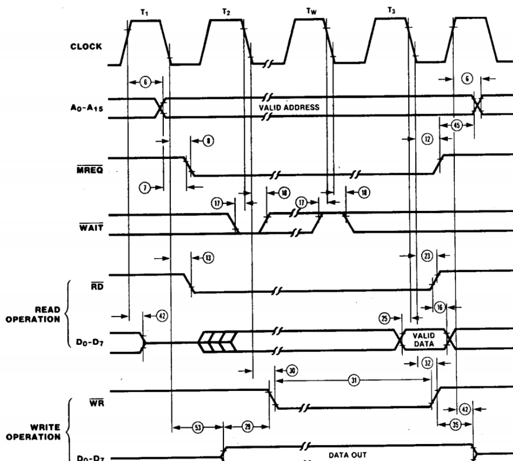
FIGURA 3-31 - MEMORY READ OR WRITE CYCLES [19]
